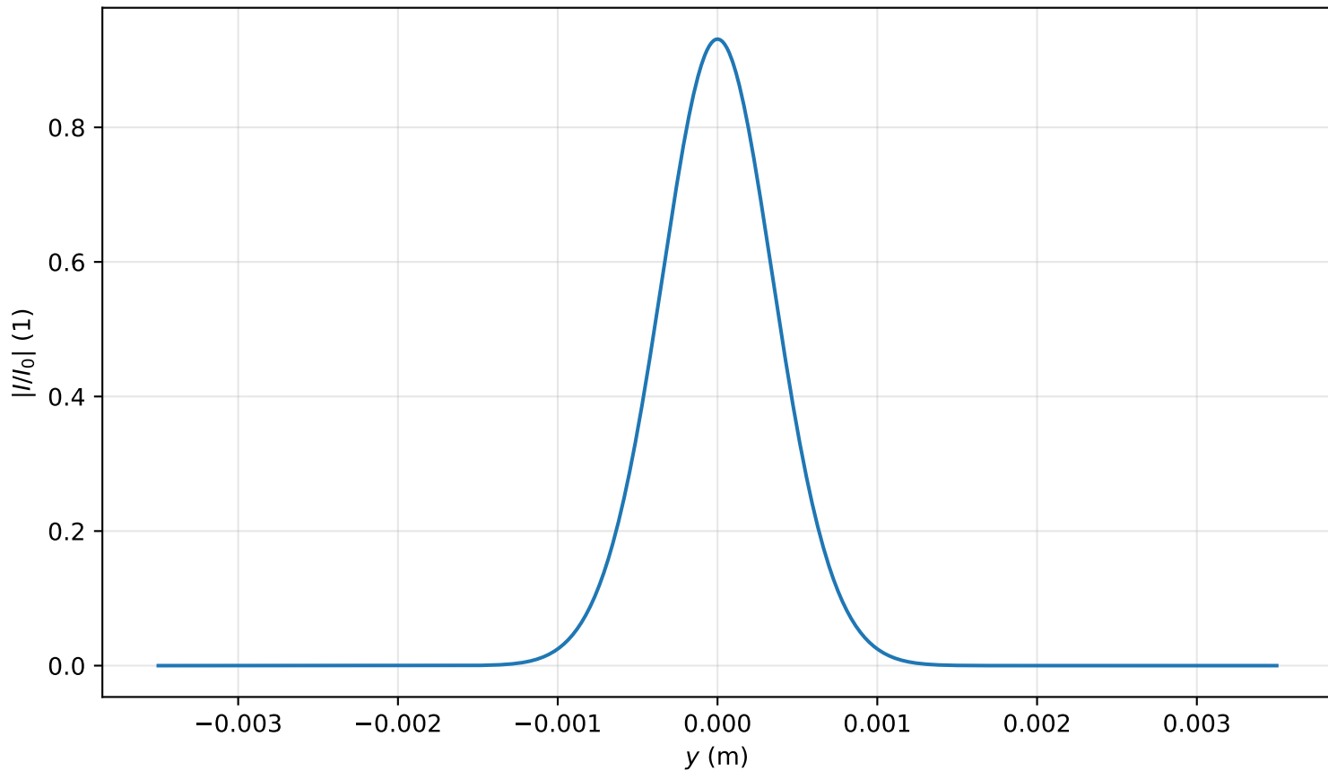
Intensity profile I(x=0, y, z=0.796)/I_0 , P_{in}=0.2P_{cr} , artificial time
